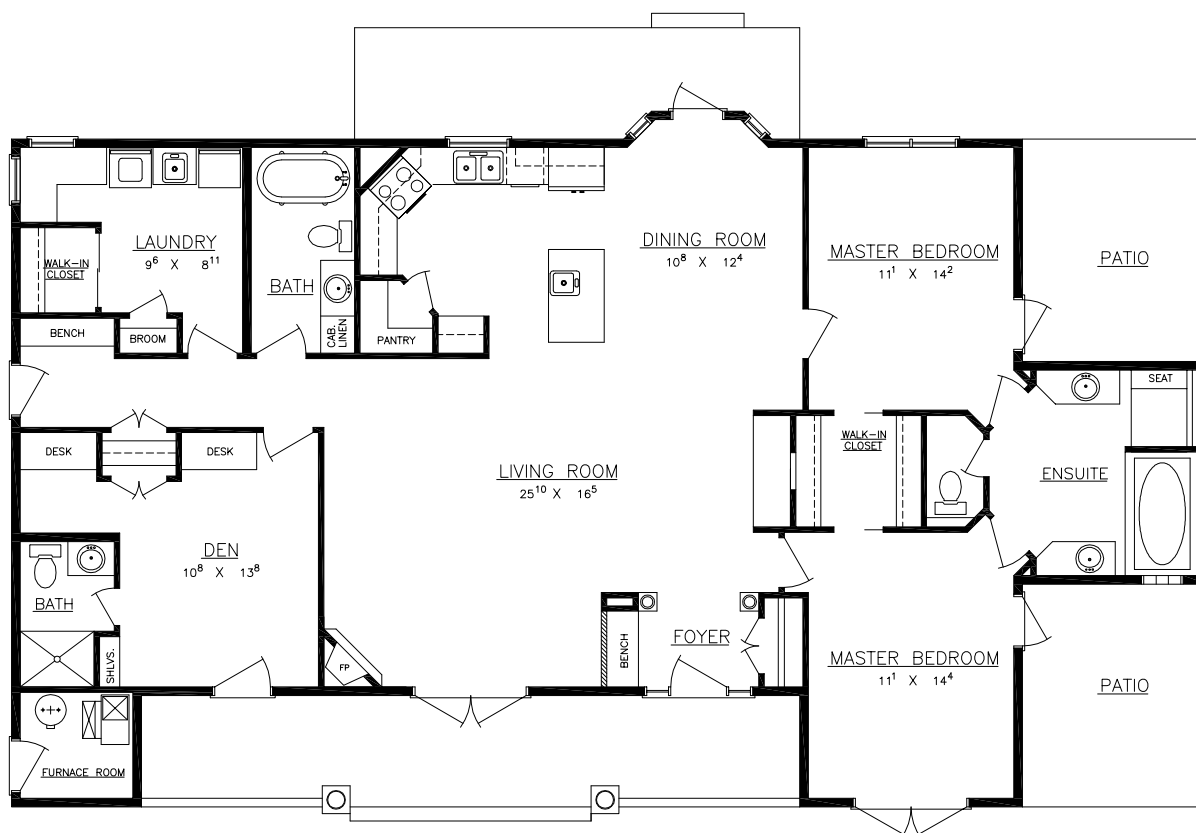
FLOOR PLAN
